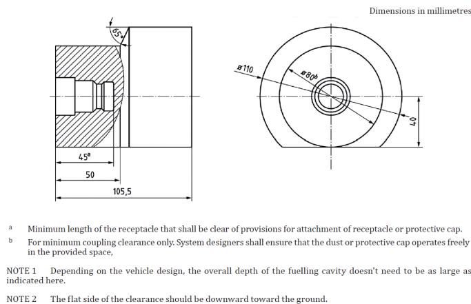
Figure 2: Screenshot of ISO 17268 with receptacle/nozzle interface envelope
